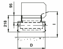
VISTA DA B VIEW FROM B
